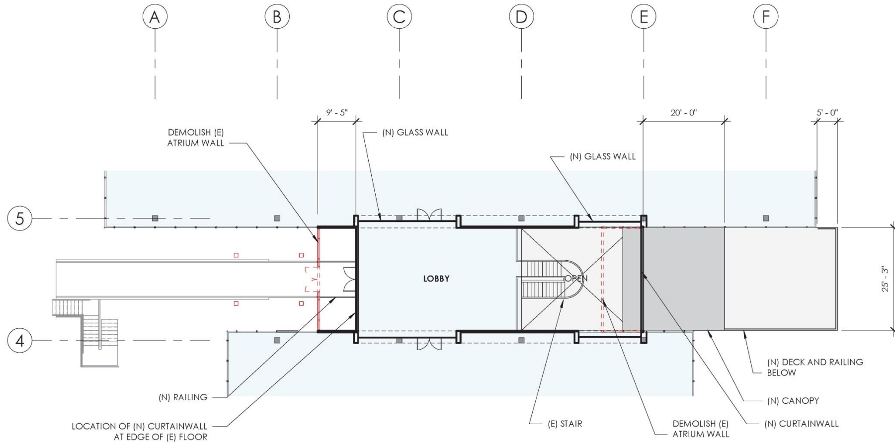
UPPER LEVEL ATRIUM PLAN
